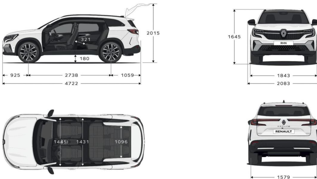
Dimensions (mm)
